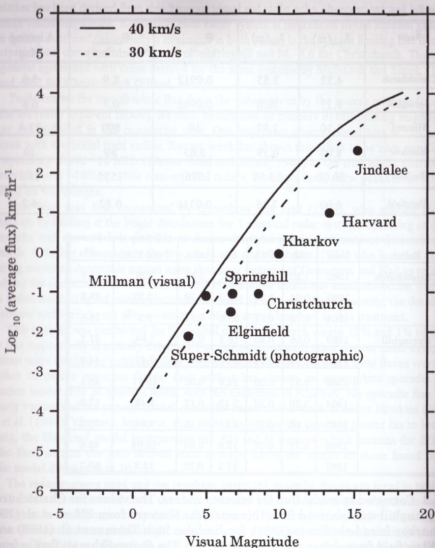
Figure 9. Raw (uncorrected) radar meteor flux as a function of equivalent magnitude. The lines are from Grün et al. (1985) and represent the transformation of the mass flux derived from impact experiments in space given in that reference to equivalent magnitudes for assumed velocities of 30 and 40 km/s using the magnitude-mass-velocity relations from Verniani (1973). Note the poor correspondence between the individual fluxes (labelled points) and the curves. These data points do not follow any logarithmic relation and particularly underestimate the flux at high magnitudes (small masses).
